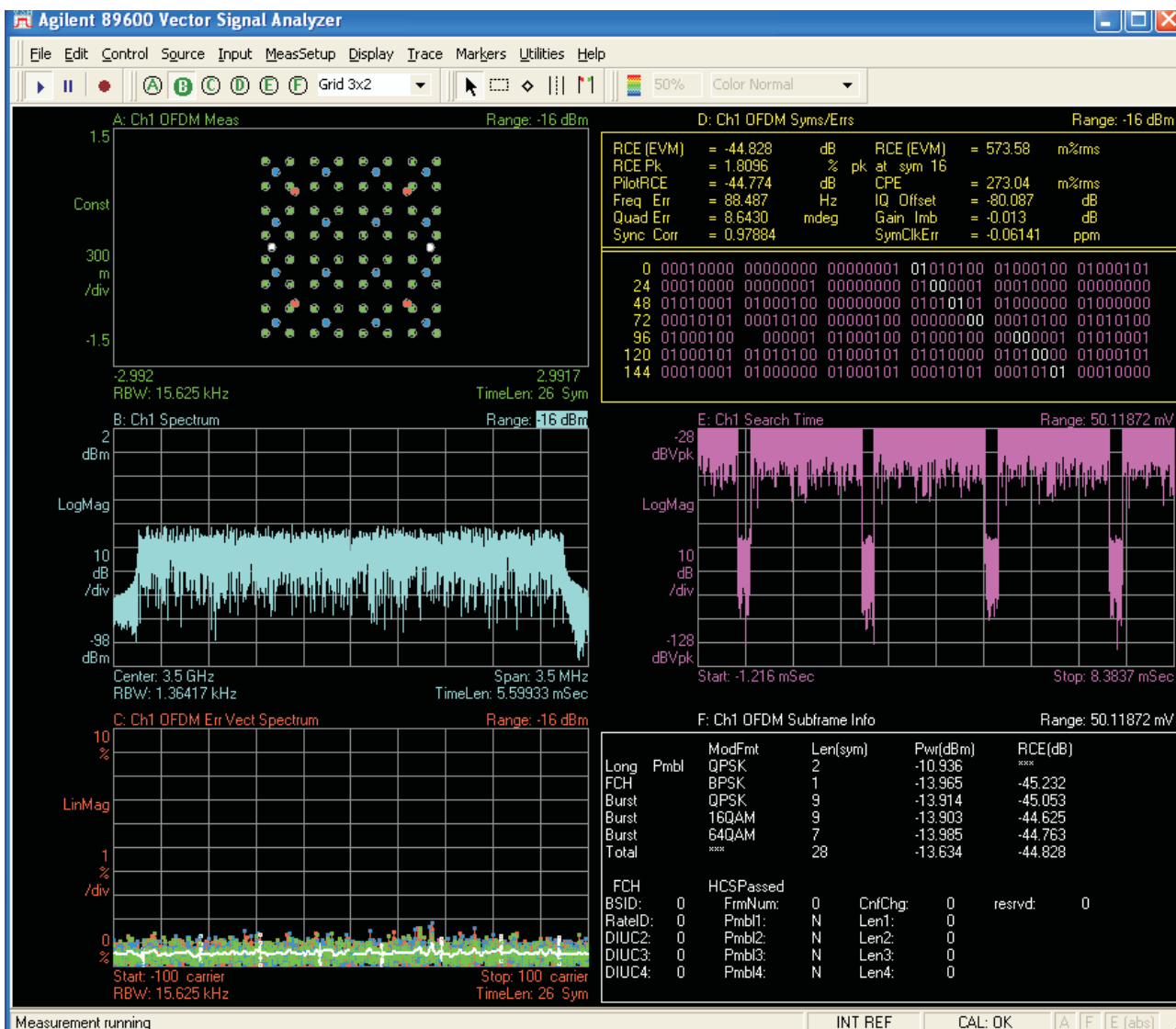
Figure 3. TRF1x22EVM Performance
